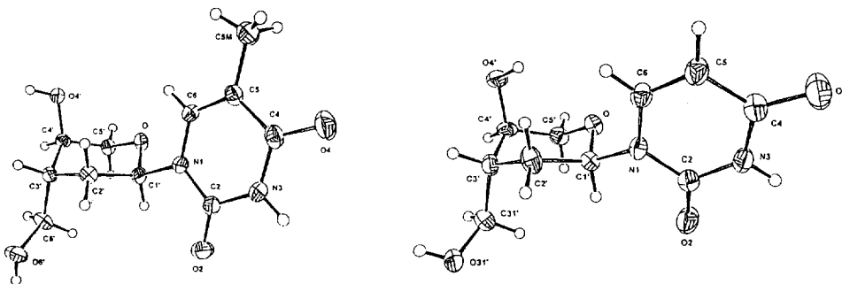
Scheme 5 : ORTEP drawing of the thymine compound 22A and the uracil compound 22B
